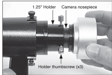
Figure 3. Insert the autoguider nosepiece about halfway into the 1.25" holder of the Mini Guide Scope, then lightly tighten the three thumbscrews on the holder to secure the camera in place for the moment.
