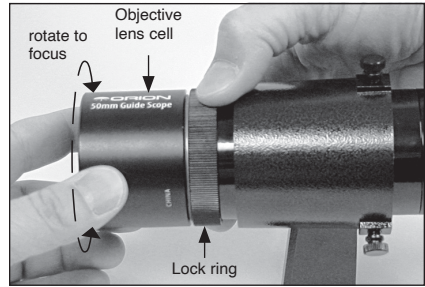
Figure 4. After setting the coarse focus with the camera in the guide scope holder, fine focusing can be done by rotating the scope's objective lens cell. First, you'll need to loosen the lock ring by rotating it counterclockwise a couple of turns.
